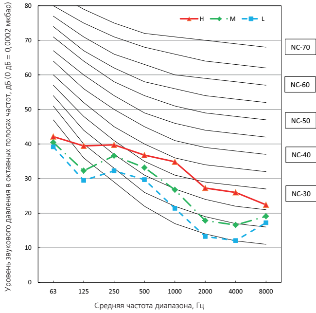
MCA3I-07NXD0, MCA3I-09NXD0
