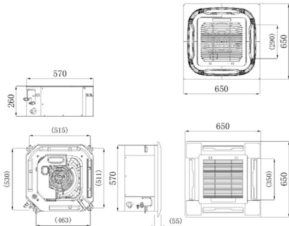
RAM-I-OK35HP.C01/S, RAM-I-OK55HP.C01/S
