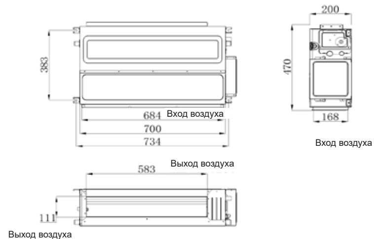
RAM-I-OK30HP.D01/S, RAM-I-OK35HP.D01/S
