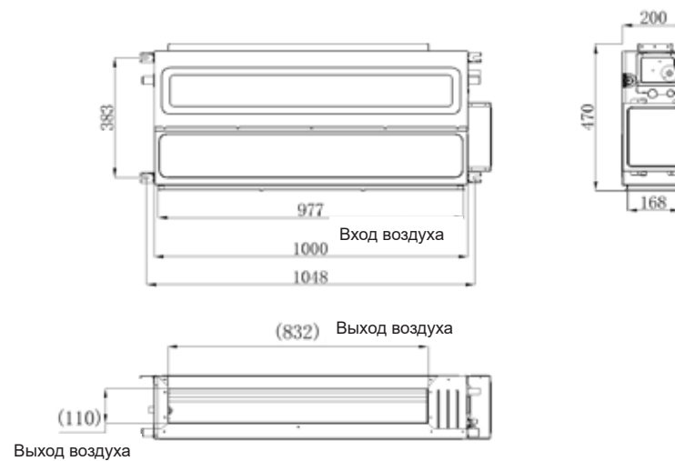
RAM-I-OK55HP.D01/S
