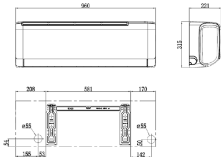
RAM-I-OK35HP.C01/S, RAM-I-OK55HP.C01/S
